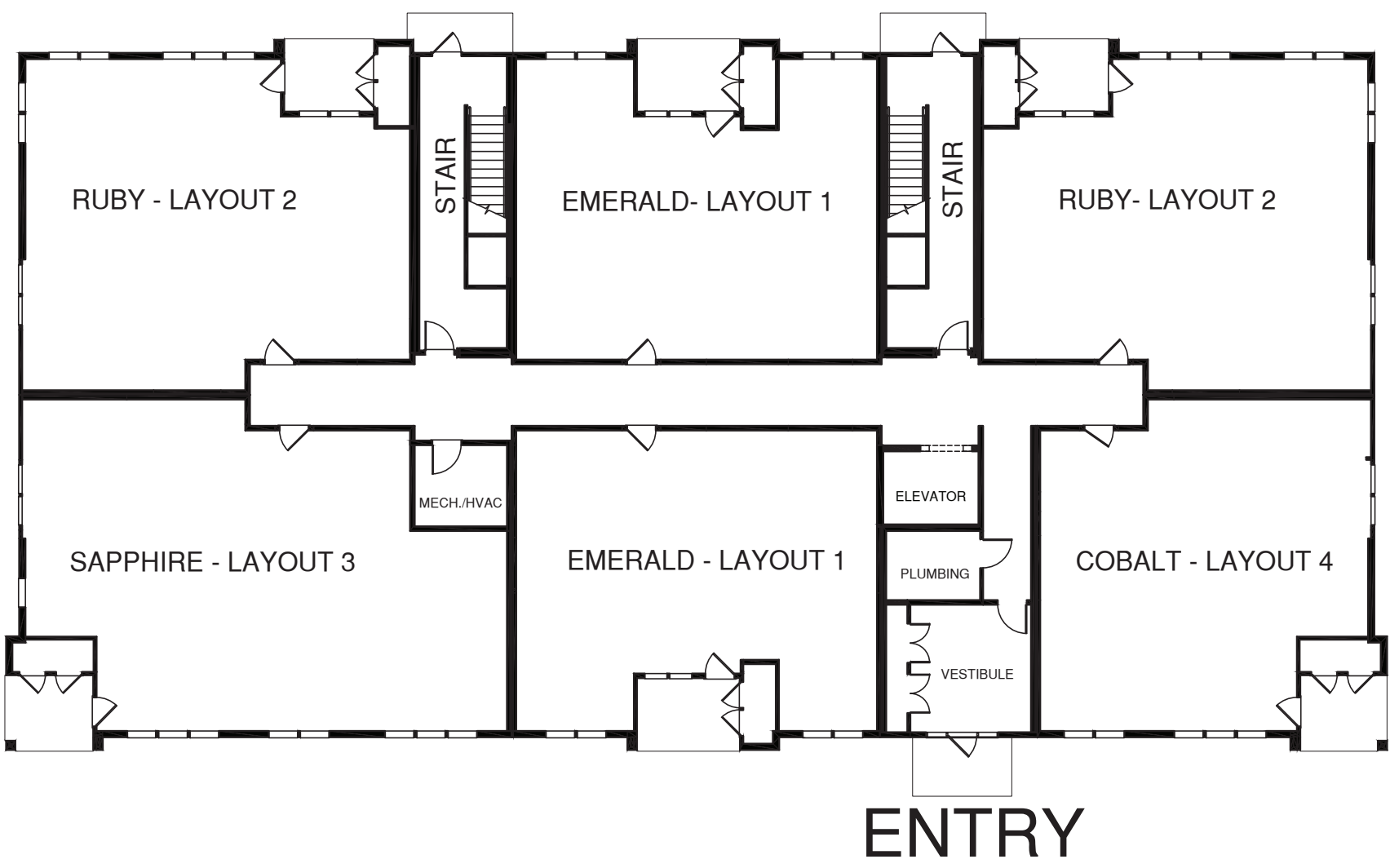
GROUND LEVEL
